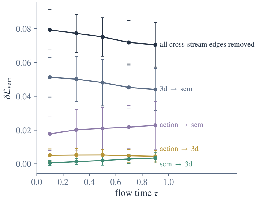
(b) the same removals, resolved in \tau
