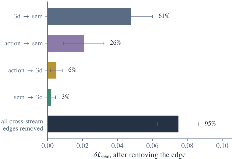
(a) edge removal, averaged over \tau (full model \mathcal{L}_{\text{sem}} = 0.0785 )
