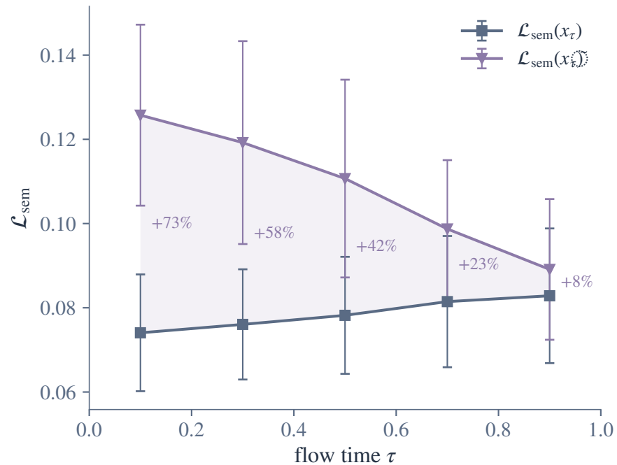
(b) future-semantics loss, true vs permuted actions
