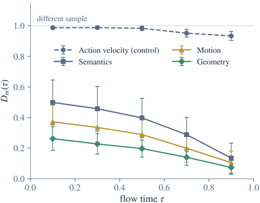
(a) representation shift under action permutation
